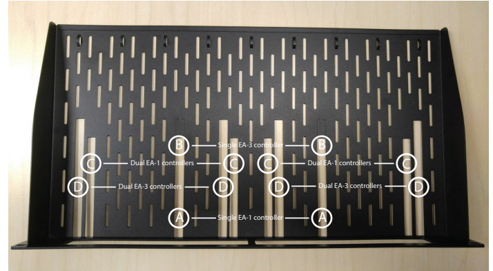
Figure 1: Rack-Mount Kit Installation Pattern Guide
